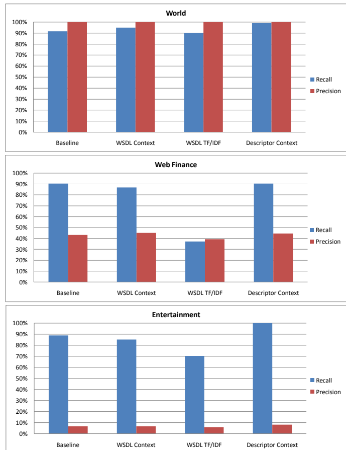
Fig. 11. Precision and Recall of All Methods
