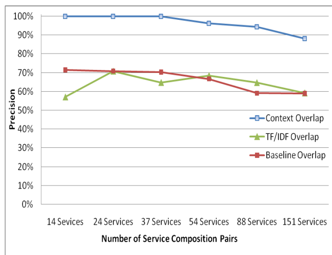
Fig. 13. Precision of Service Matching According to Contextual Ranking
