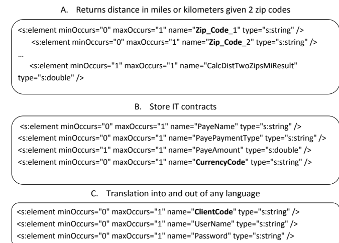
Fig. 1. Service Tagging is Misleading: an Example
